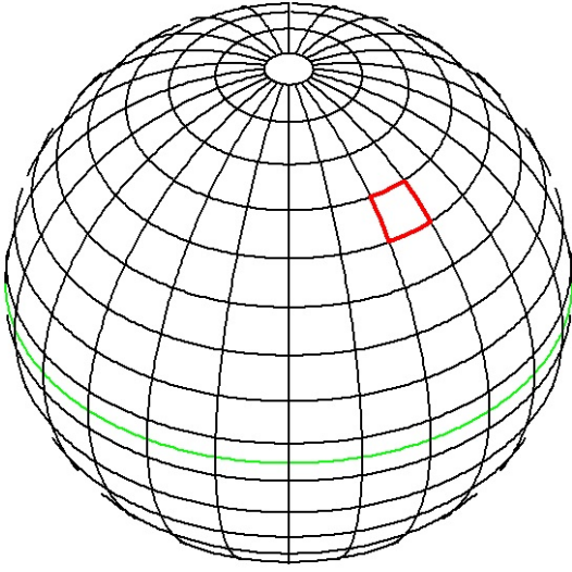
Fig. D.1. The partition of directions into 10 x 15 deg ( \theta , \phi ) quads as used in HydroLight. The green line is the “equator” dividing upward and downward directions. The red quad illustrates where the sun might be placed for a zenith angle of 40 degrees.
